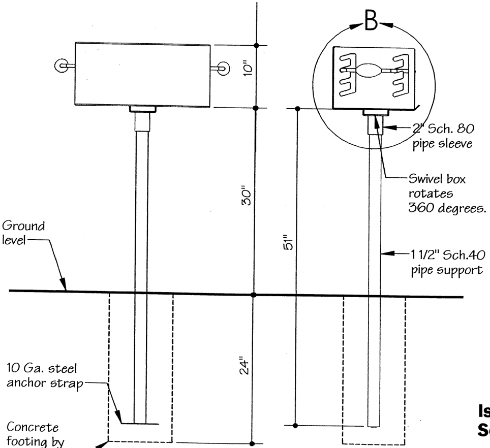
Elevations
