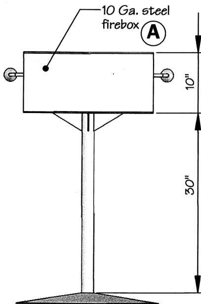
Elevations
