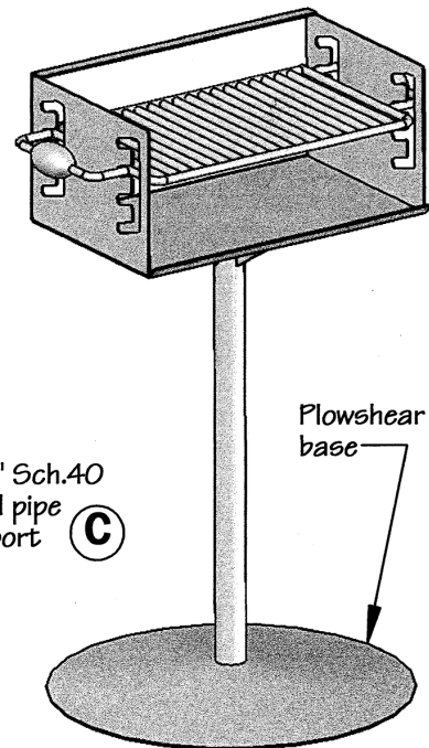
Isometric View of Freestanding Barbecue
