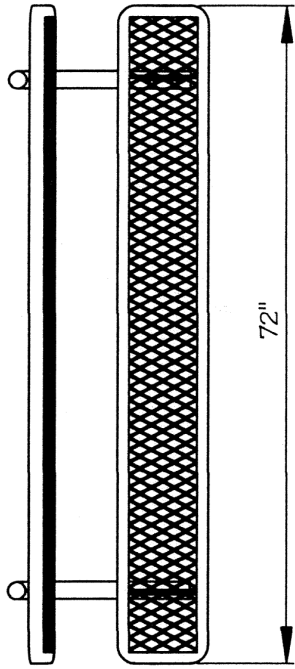
PLAN VIEW
