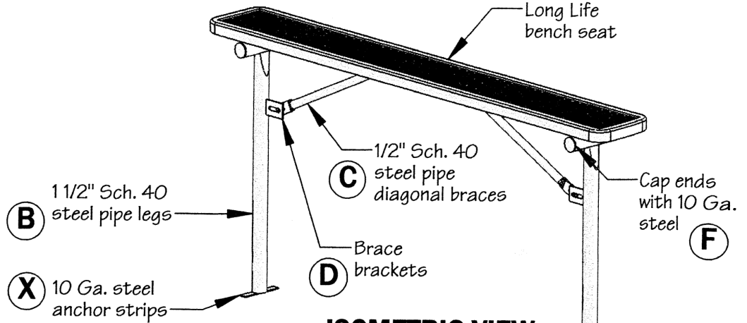
ISOMETRIC VIEW of SOLID MOUNT PARK BENCH - NO BACK
